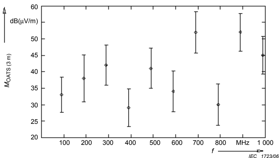
Figure B.22 – Sample OATS (3 m) measurement
