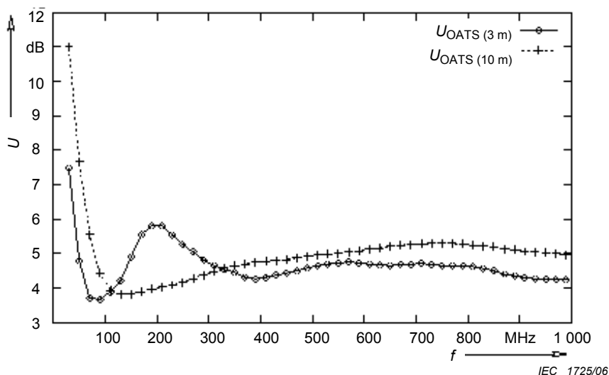
Figure B.24 – Expanded uncertainties
