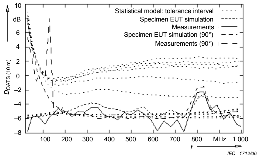
Figure B.11 – Deviations of the specimen EUT: 3 m fully anechoic room (top) and 10 m open area test site (bottom)
