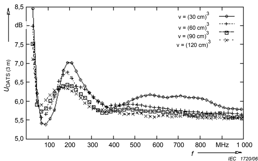
Figure B.19 – Expanded uncertainties ( k = 2 ) of alternative test method [OATS (3 m)]
