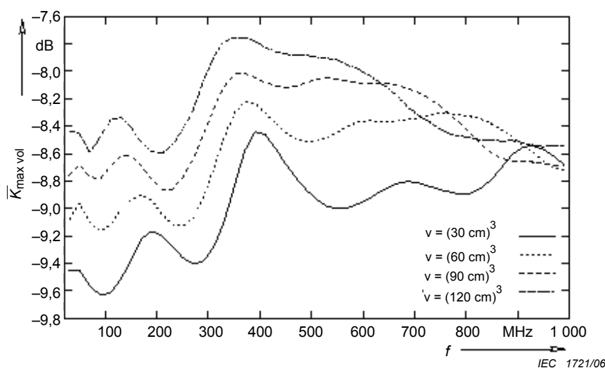
Figure B.20 – Maximum average conversion factors
