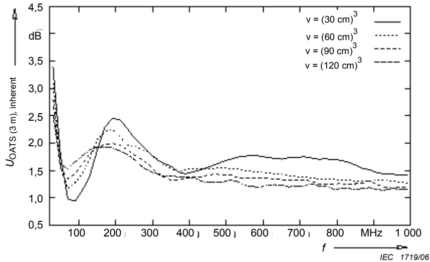
Figure B.18 – Uncertainties due to the unknown EUT characteristic for 3 m OATS
