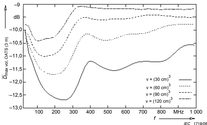
Figure B.17 – Maximum average deviations for 3 m OATS
