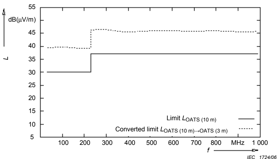
Figure B.23 – OATS (10 m) limit line converted to OATS (3 m) conditions
