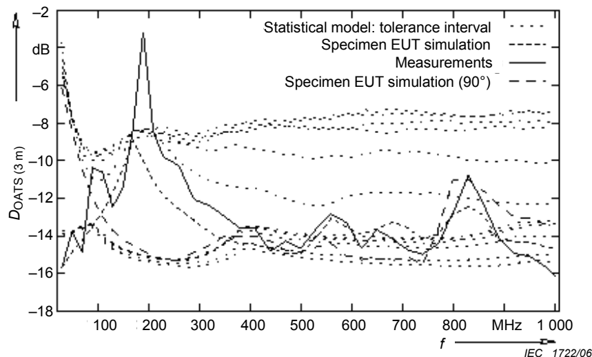
Figure B.21 – Deviations of the specimen EUT: Open area test site (3 m)
