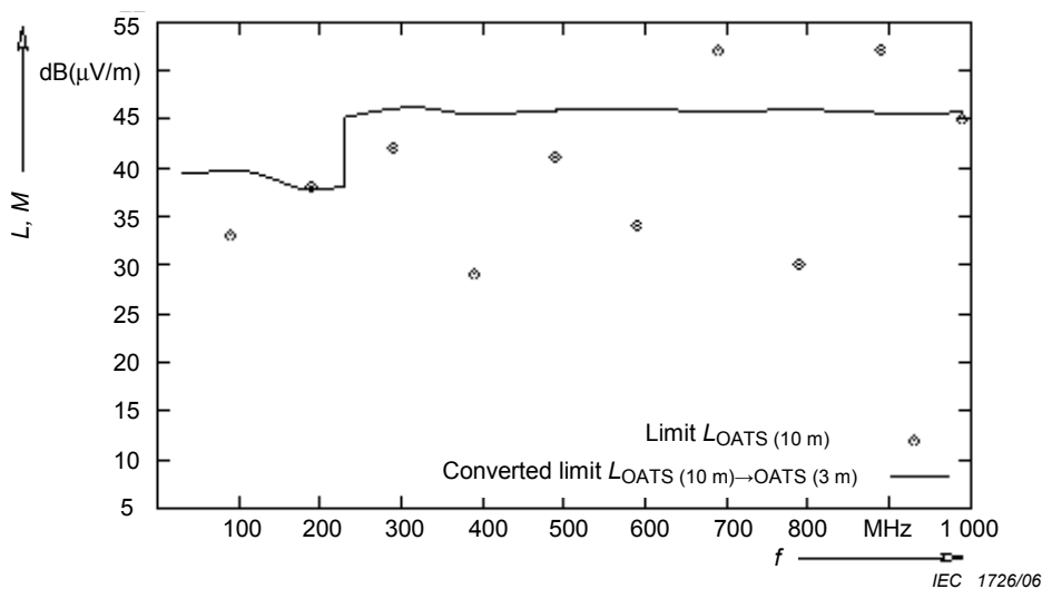
Figure B.25 – Comparison of the corrected values with the converted limit
